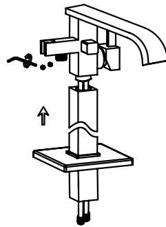
5. Tighten up the pipe to the body with H2.5 hex key.
