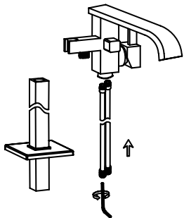
4. Connect body by H8 screw tool, install the decorative cover from top of the pipe, tighten up inlet pipe to the body with H8 hex key.
